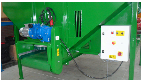
conveyor belt with steering ropes and standard fixed speed
